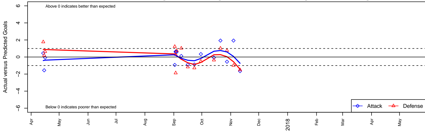
Coastal FC B01 Dots are actual minus expected GF (blue circles) and GA (red triangles). Blue line is smoothed change in attack strength. Red is smoothed change in defense strength.
